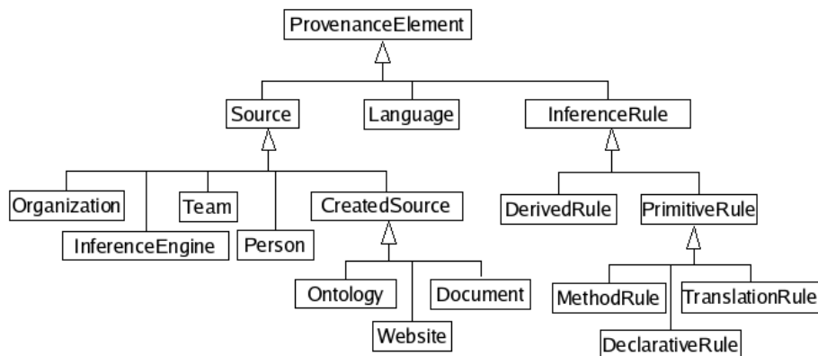
Figure 2: Top of the PML taxonomy of provenance elements.
